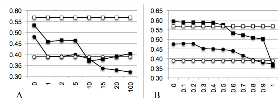
Figure 2. A: Tuning of the cost injection. B: Tuning of the resistance profile injection. Axis x represents the value assigned to the data without injection information and axis y represents the top precision. Baseline top-precisions are represented with ○ for easyIR and □ for PubMed. Multimodal re-ranked top-precisions are represented with ● for easyIR and ■ for PubMed.
